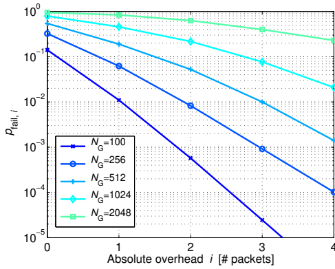
Figure 10: Decoding performance of systematic RLNC over erasure channel with 40% packet loss rate.
