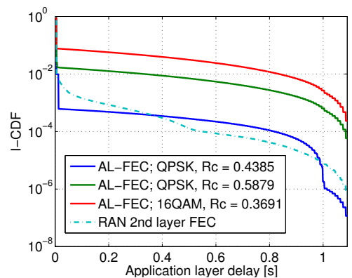
Figure 18: I-CDF of application layer packet delay for AL-FEC with various MCS settings and for 2nd layer of FEC with 'QPSK, R_c = 0.59 '.
