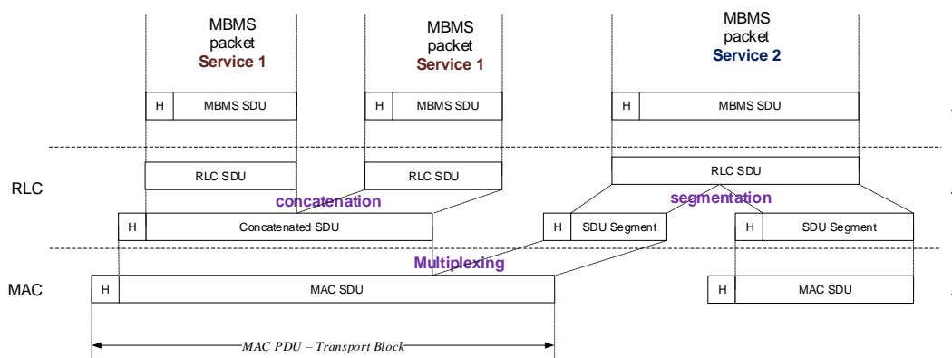
Figure 2: Packet flow for MBMS data [5].
